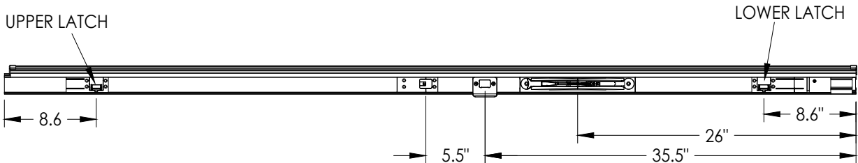
HARDWARE LOCATIONS
