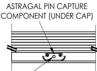
DETAIL 2 Inswing Articulating Threshold
