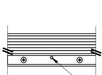
DETAIL 2 Inswing Adjustable Threshold
